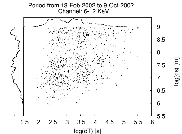
Figure 1. The distribution of succeeding flares in the \{\log_{10}(ds); \log_{10}(dT)\} plane. Note the two major populations of the events divided by a horizontal "valley" at about 10^8 m. The rising trend in the lower population of events may indicate some relationship between the temporal and spatial differences of succeeding flares.
