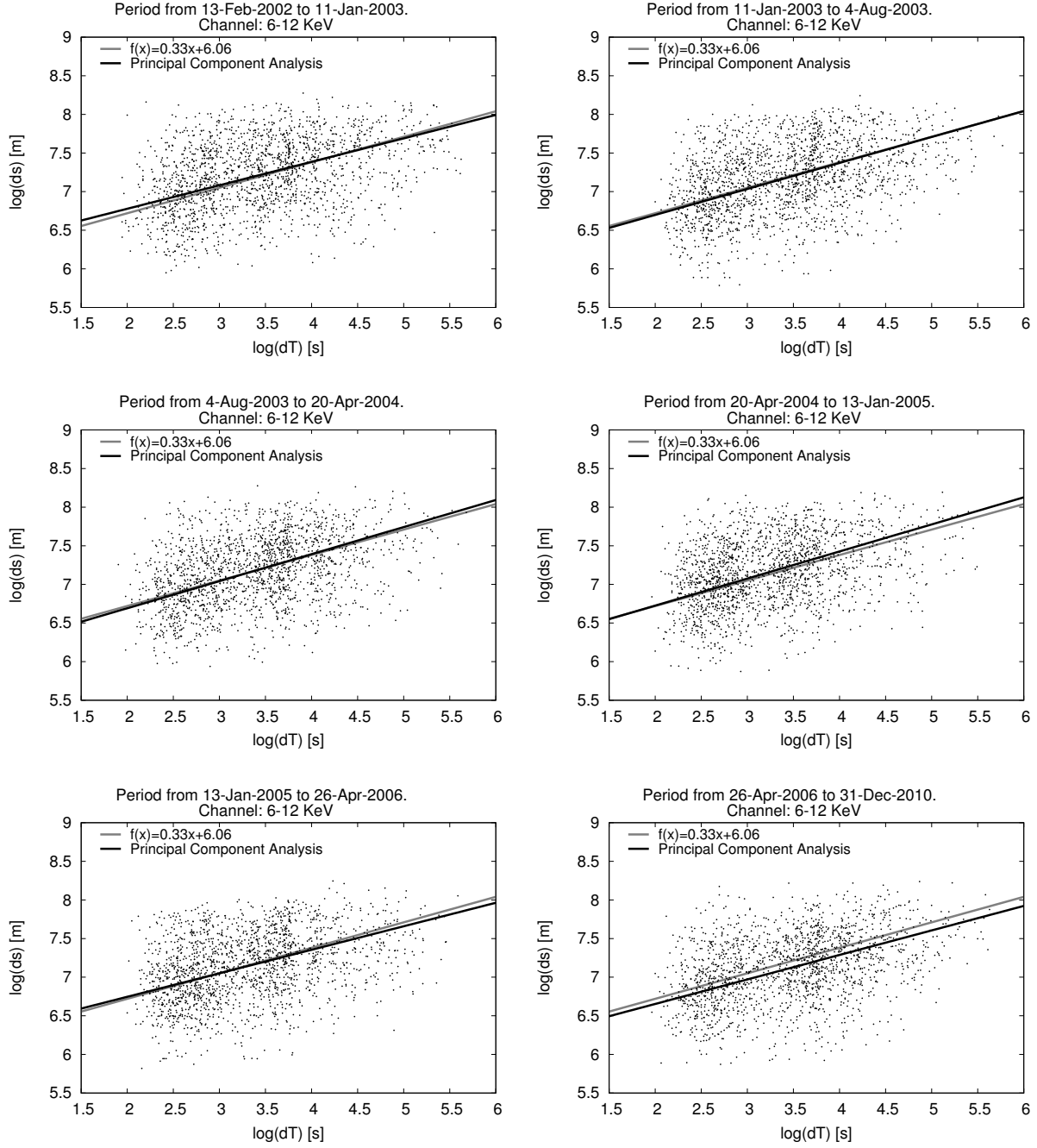
Figure A1. Distribution of flares measured in the 6-12 keV channel and their successors in the \{\log_{10}(ds); \log_{10}(dT)\} plane. The black solid line indicates the actual result of the PCA regression and the grey line is determined by the average parameters in Table 2.
