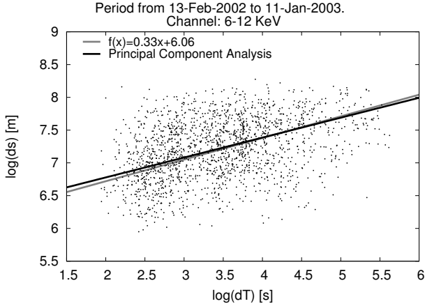
Figure 2. Distribution of flares in the 6-12 keV channel and their successors in the \{\log_{10}(ds); \log_{10}(dT)\} plane. The black solid line indicates the actual result of the PCA regression and the grey line is determined by the average parameters of Table 2.
