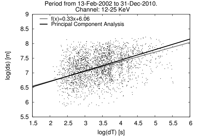
Figure 3. Distribution of succeeding flares in the \{\log_{10}(ds); \log_{10}(dT)\} plane in the 12-25 keV channel. The meaning of the lines is the same as in Figure 2.
