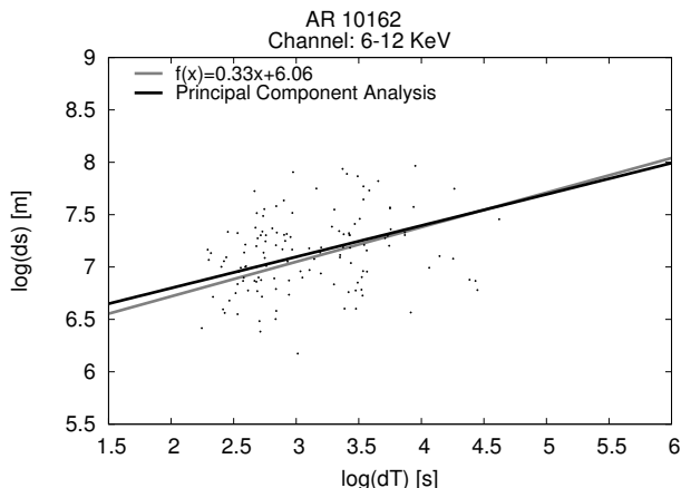
Figure 4. Distribution of succeeding flares in the \{\log_{10}(ds); \log_{10}(dT)\} plane in the 6-12 keV channel for the active region AR 10162. The meaning of the lines is the same as in Figure 2.
